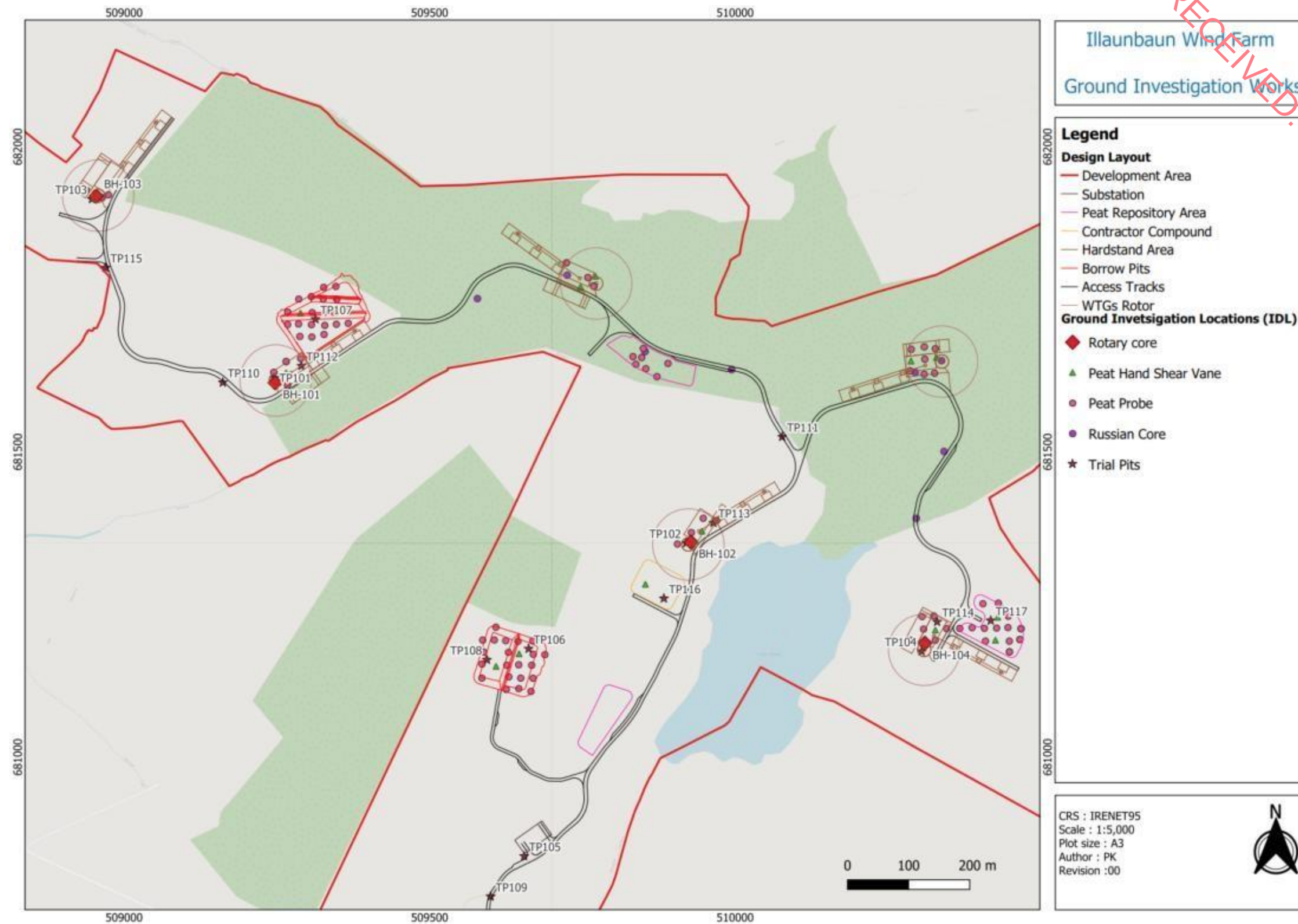
Figure 3-1: Ground investigation works completed by IDL (2024)
