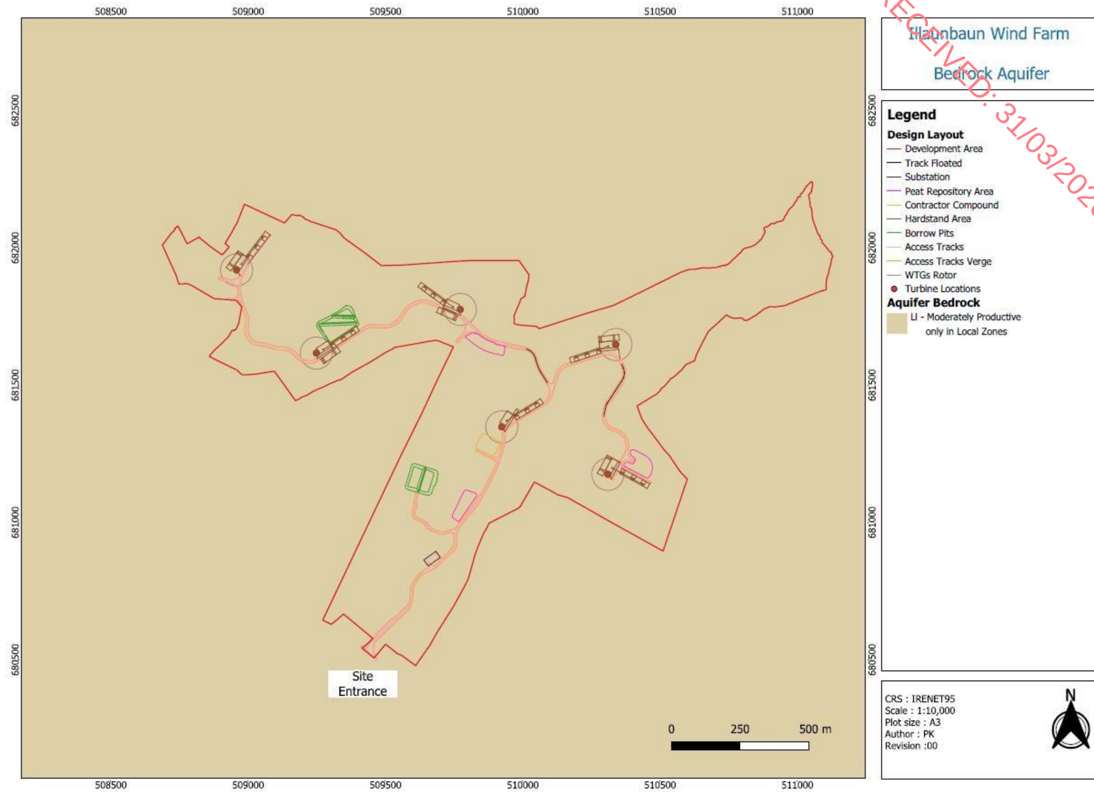
Figure 2-5: Bedrock Aquifer
