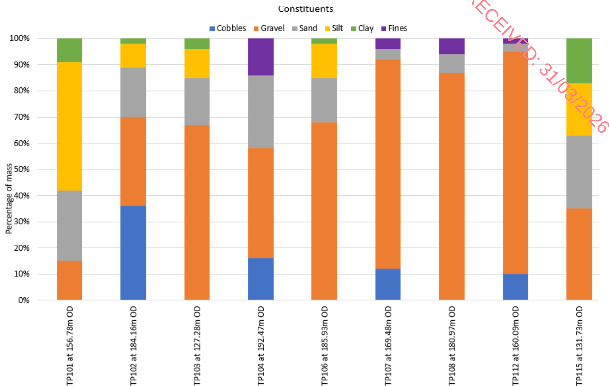
Figure 5-2: PSD fraction distribution
